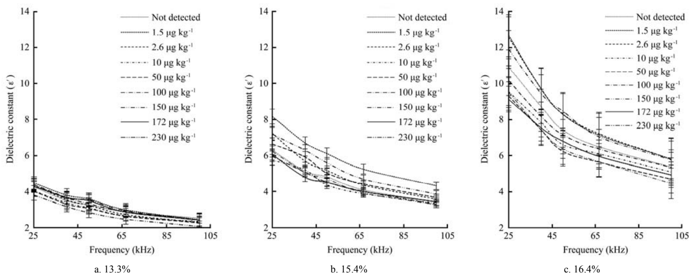
Figure 2 Variation of dielectric constant with frequency at specified aflatoxin levels for maize kernels at m.c. (w.b) ( \text{LSD}_{p<0.05} = 0.3154 , \text{CV} = 0.014 )
