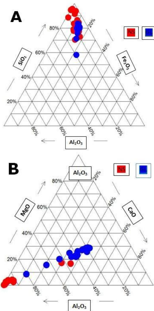
Fig 2: Distribution of (A) dominant oxides (B) dominant neutralizing oxides and acid-forming oxide in Nestor (NS) and Glynn Lydenburg (GL) mine tailings
