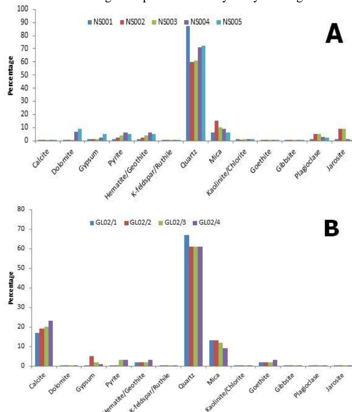
Fig 3: The mineralogical analysis of (A) Nestor and (B) Glynn Lydenburg mine tailings
