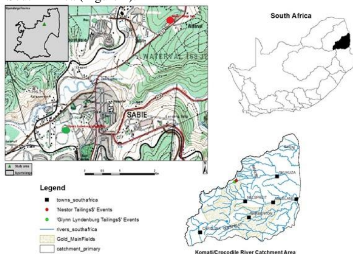
Fig 1: The location of mine tailings in Mpumalanga province, South Africa
